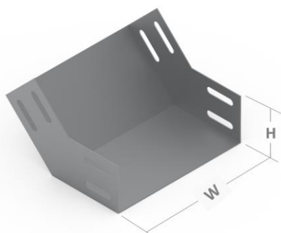
Curva horizontal 45° Ref. 1019
