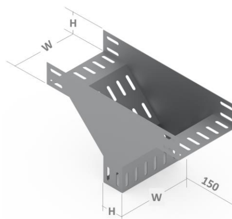
Tê vertical de descida Ref. 1032
