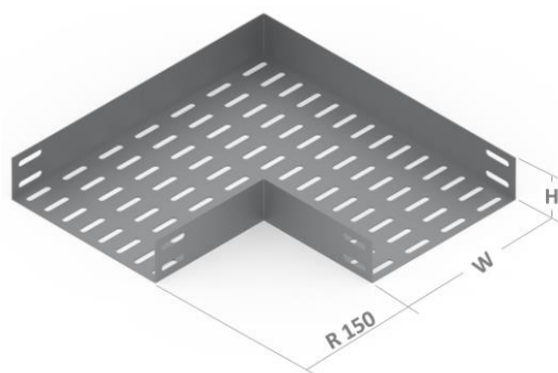
Cotovelo Reto Ref. 1020
