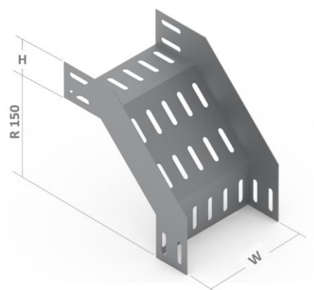
Curva vertical externa 90° Ref. 1013
