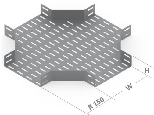
Cruzeta horizontal 90° Ref. 1025
