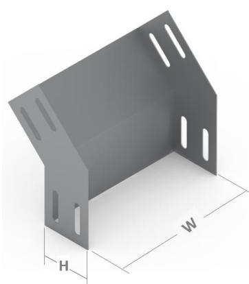
Curva vertical externa 45° Ref. 1014
