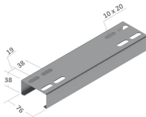
Perfilado liso 19x38 Ref. 2008
